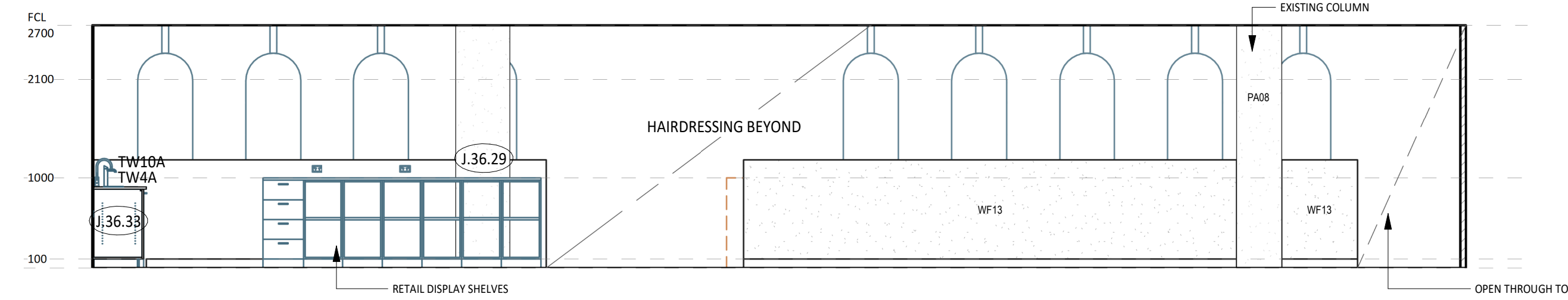
2 ELEVATION DETAIL 1 : 50
